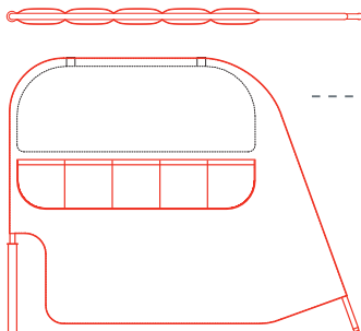
Backbone for high screen 1BE0201 : L 80¾ D 2½ H 63
