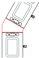
"V" shaped connector for backbones 1BE0256 : L 19 D 12¼ H 21
